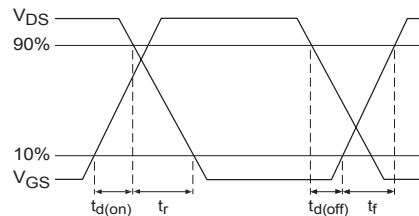
Fig 10b. Switching Time Waveforms
